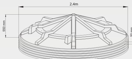
Roofs nest together for transport (approximately 40kg per roof) Allow 50mm for every additional roof in the stack
