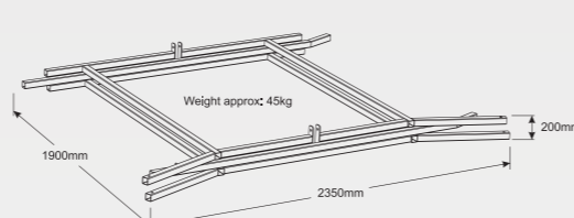
Frames flat pack for transport (approximately 68kg per frame)
